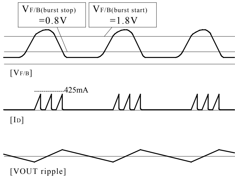
Fig.3 Standby Operation Sequence
