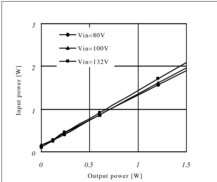
Fig.9 Standby Power Consumption
