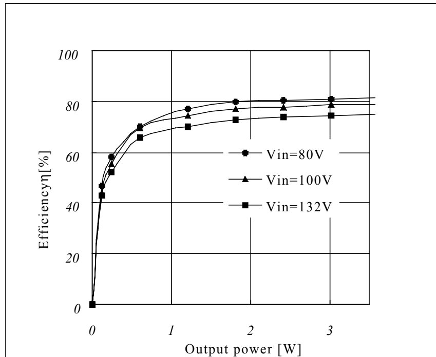
Fig.8 Efficiency Characteristics (standby)
