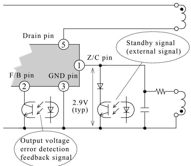
Fig.2 Standby Mode Selector Circuit
