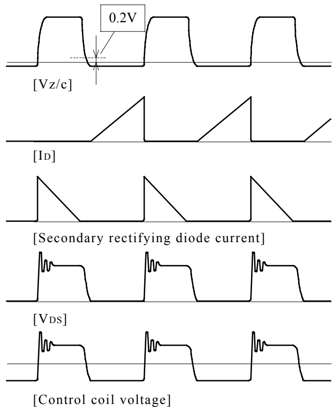
Fig.1 ON Trigger Operation Sequence
