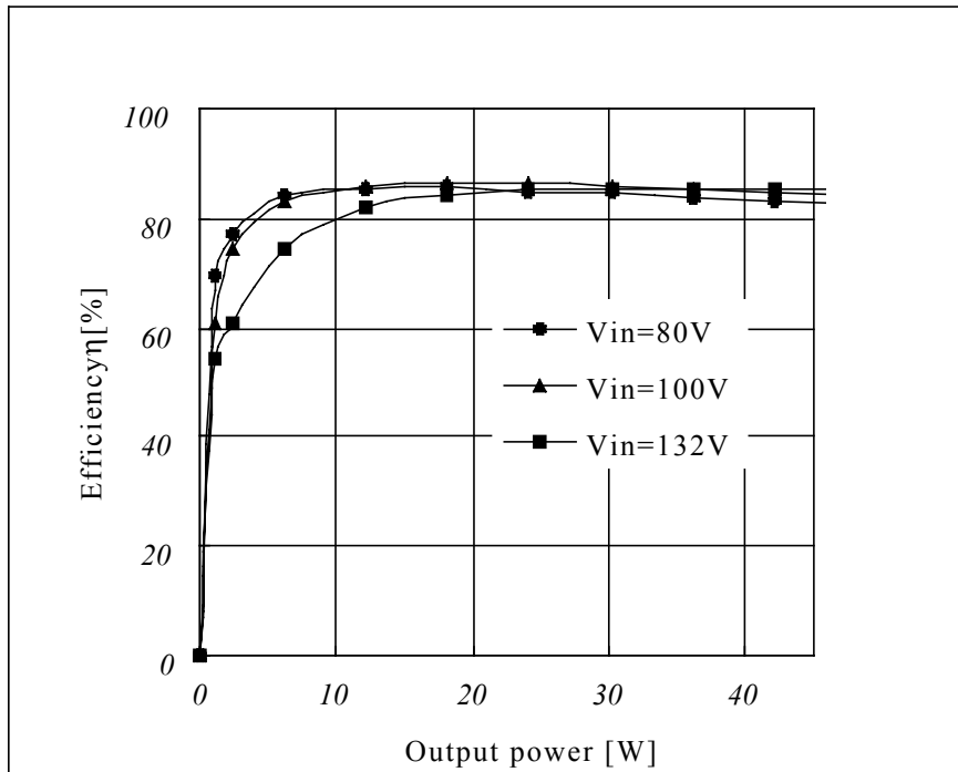
Fig.7 Efficiency Characteristics (steady-state)
